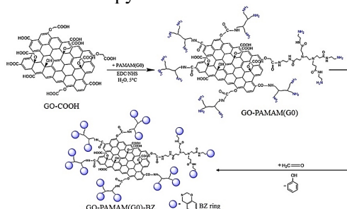
Fig. 1. Hyperbranched benzoxazine functionalized graphene oxide (GO-PAMAM-BZ)
