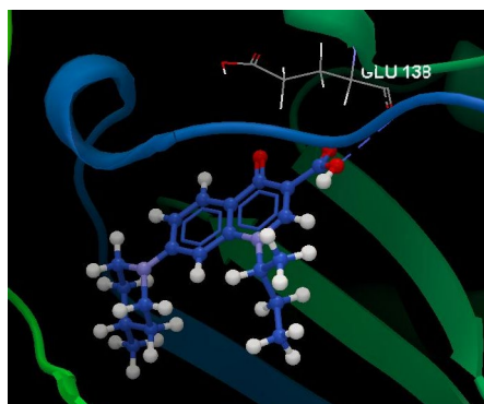
Figure 1. Hydrogen bond (blue dotted lines) between HPQ31 and amino acid residue from binding site of 2DZ1 receptor
