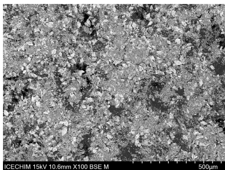
SEM image for the multilayered nanocomposite material composed of Hydrotalcite/TiO 2 /ZnHAP/Ca(OH) 2
