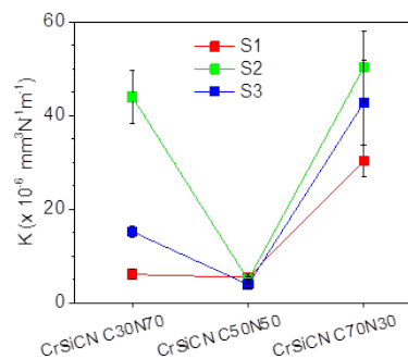
Figure 2. Wear rate, K, for CrSiCN coatings deposited on S1-S3 substrates
